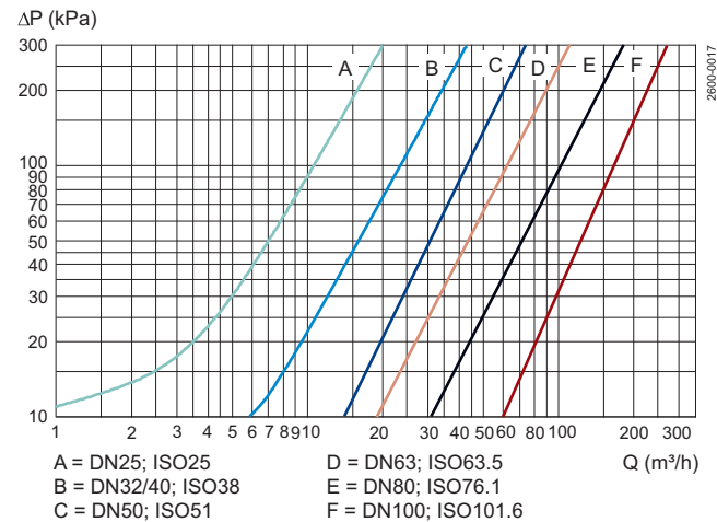
Fig. 1. Note! For the diagram the following applies: Medium: Water (20°C) Measurement: In accordance with VDI 2173.
